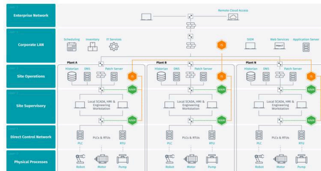
Sample OT deployment of Industrial Security (IS) consoles and NNM sensors
